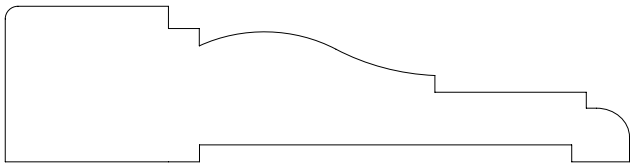
C36 - 13/16 x var to 3-1/2" □
