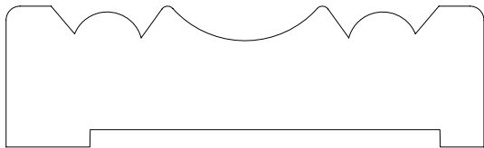
C80 - 13/16 x 2-3/4" □
